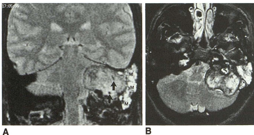
Fig. 2. T2-weighted images.
