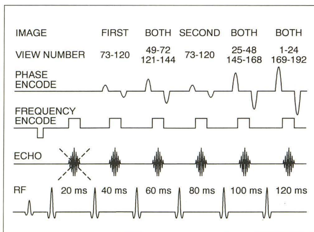
Fig. 1. Pulse sequence timing diagram for SHARE technique. The multiecho train consists of 6 echoes, formed at 20-msec intervals. The first echo is not sampled, but its formation is an important feature of SHARE.
