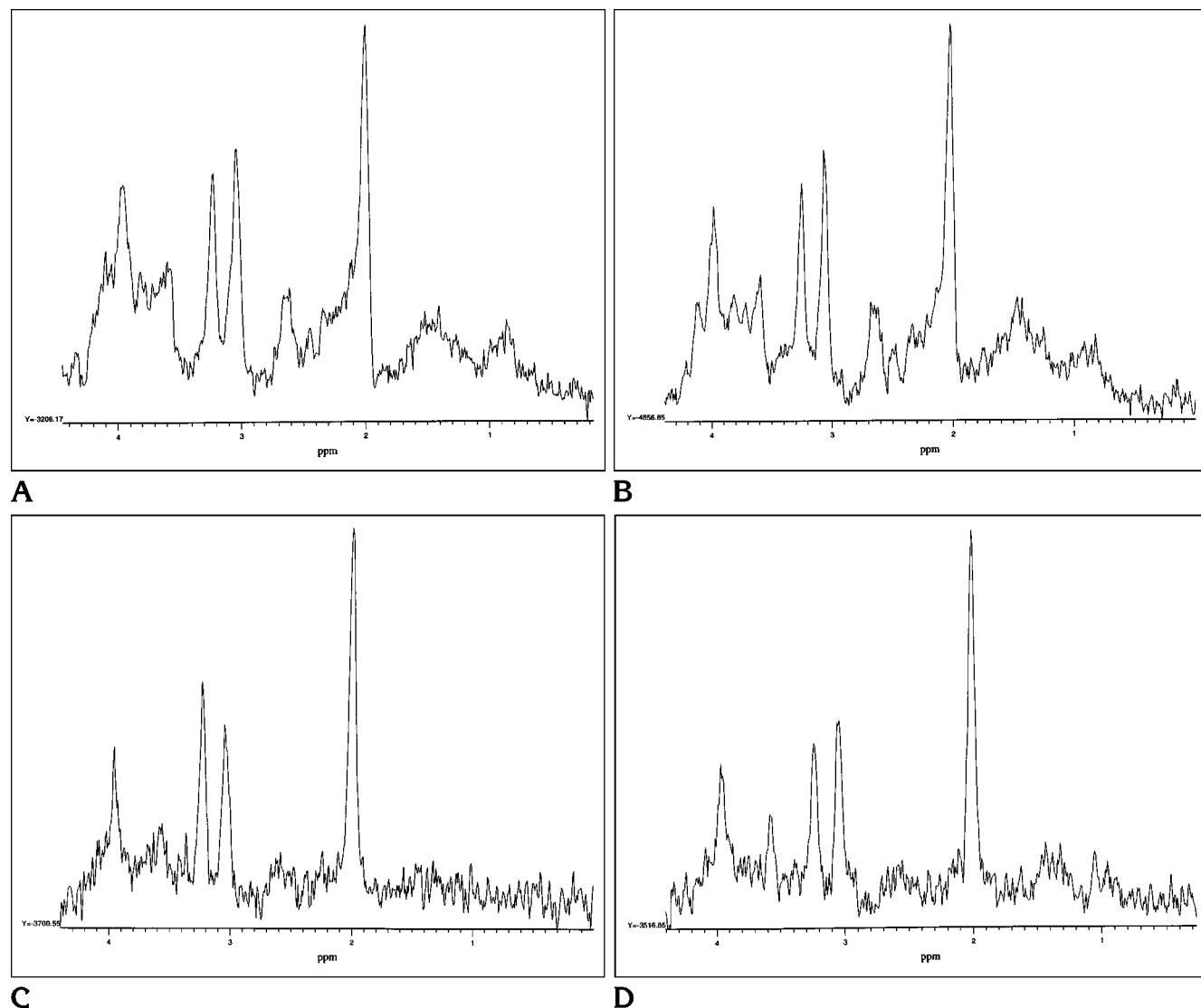
Fig 2. Representative proton MR spectra at TE 30 (A and B) and 136 (C and D) in a control subject (A and C) and the patient with severe white matter changes (patient 2, Table 1) shown in Figure 1C (B and D). Peak assignments in parts per million (ppm) are: NAA, 2.02; Cr, 3.05; Ch, 3.25; and MI, 3.6.
