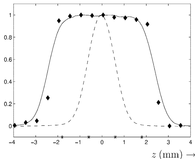
Fig 1. Section sensitivity profiles for sequential mode (diamonds) and spiral mode (dashed line). The continuous line depicts the profile of 4 combined spiral mode images with an increment of 1.2 mm (positions of each image given by asterisks on the z-axis).
